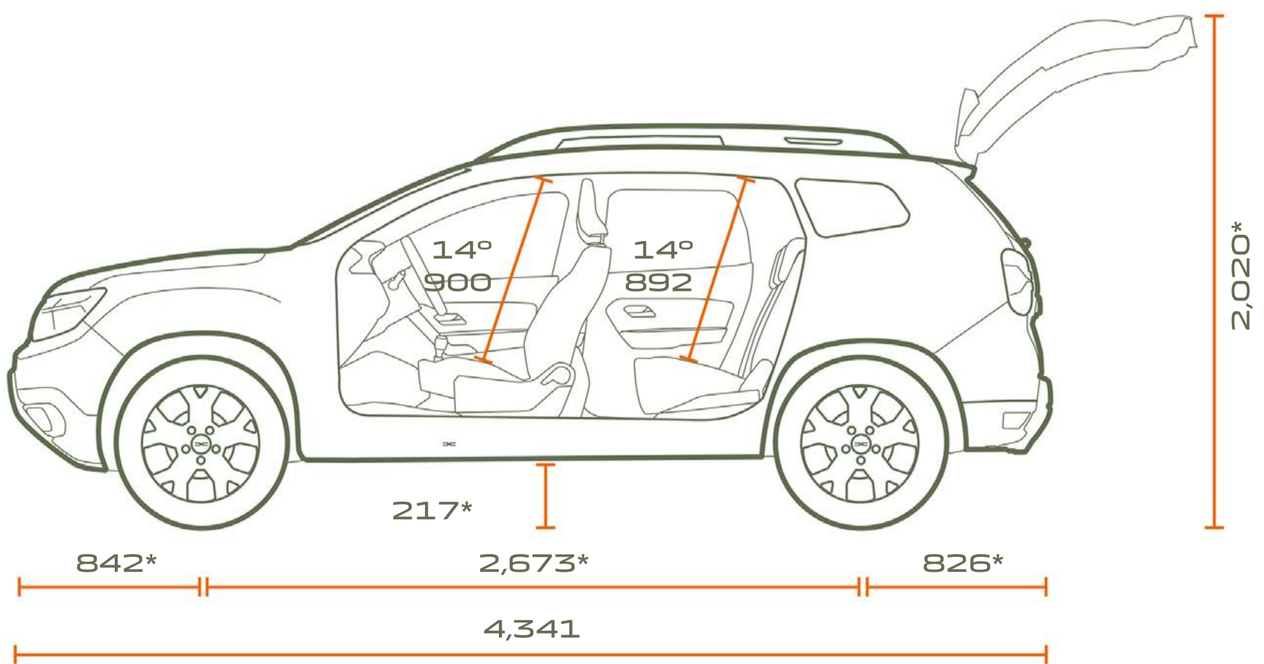
PROFILE VIEW
